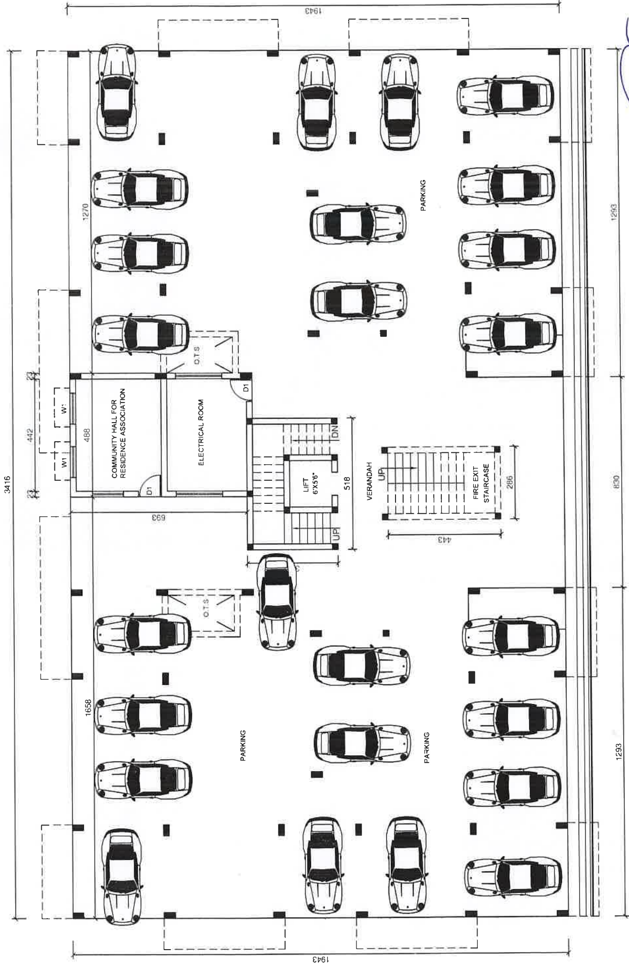
GROUND FLOOR / PARKING PLAN BLOCK - 3
