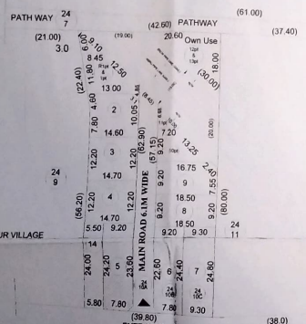
LAYOUT PLAN (1:500)
