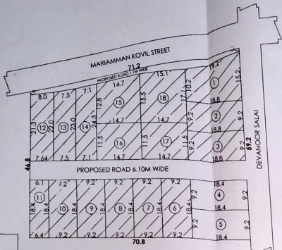
LAYOUT SKETCH (1:100)
